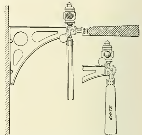
TRAIN ORDER SIGNAL USED ON E. T., VA. & GA., COLOR AND POSITION USED FOR DAY INDICATION.
